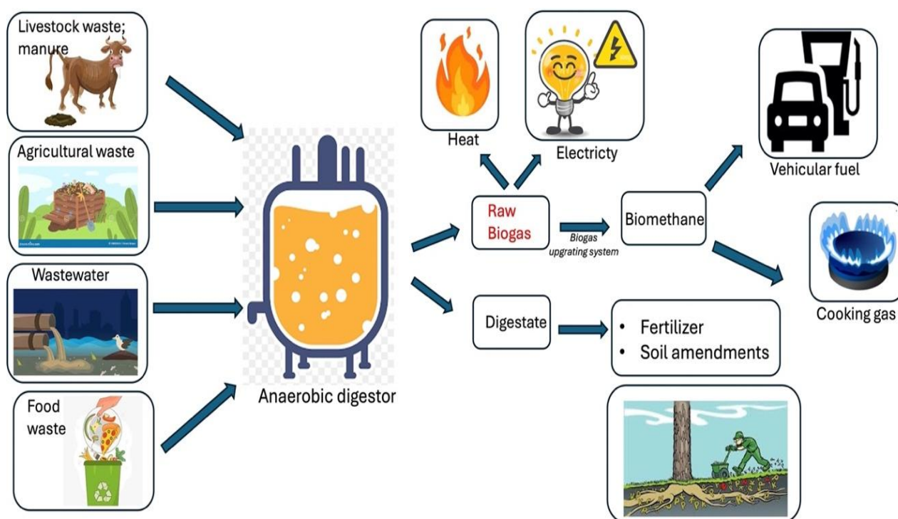
Figure 1. Schematic representation of biogas production, adapted from Upadhyav et al. (Upadhyay et al., 2023) and October 2017 EESI report ( https://www.eesi.org/papers/view/fact-sheet-biogasconverting-waste-to-energy )
